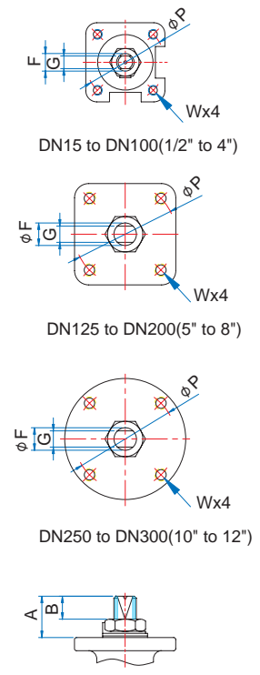
Sizes DN125 to DN300(5" to 12") optional
