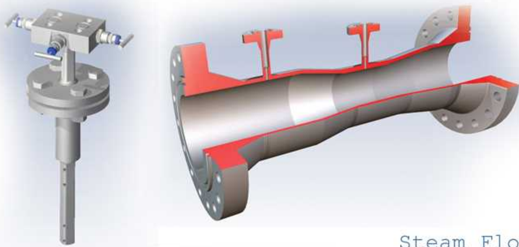
Steam Flow Meter
