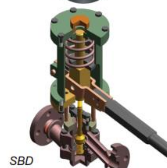
Blow Down Control Valve
