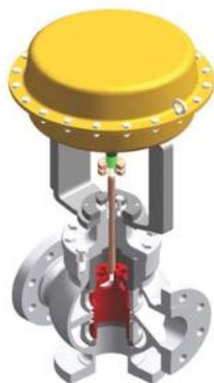
3-Way Valve
